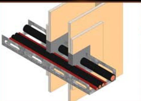
Small Cable Tray and Cables FRL-/60/60
